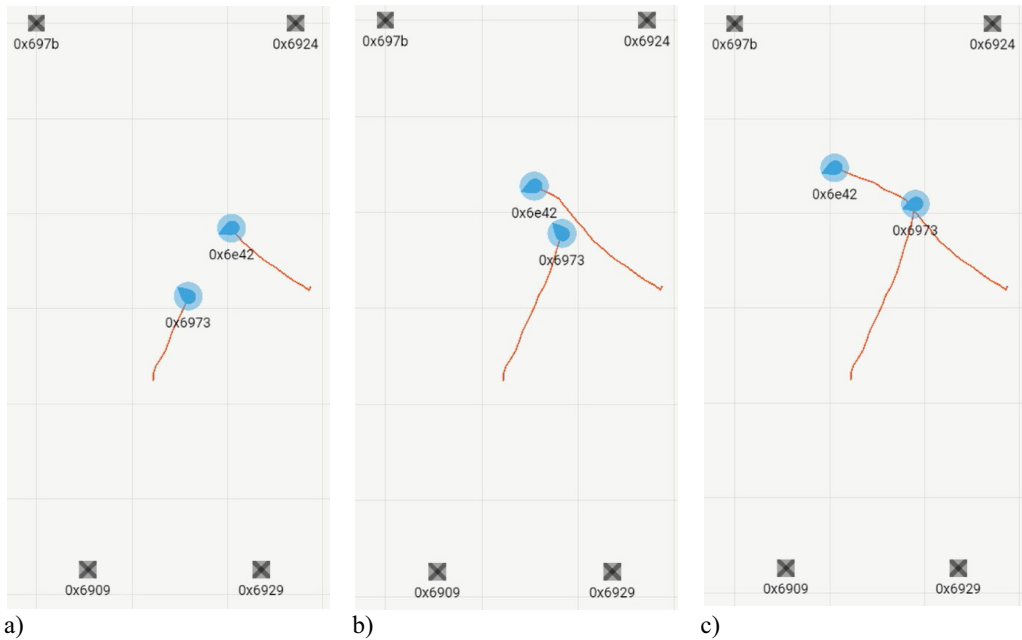
Fig. 4.6. Exemplary results of real experiments with a dynamic obstacle
